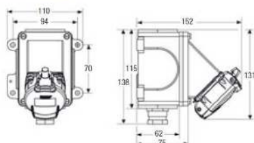
Socle mural (45°)
